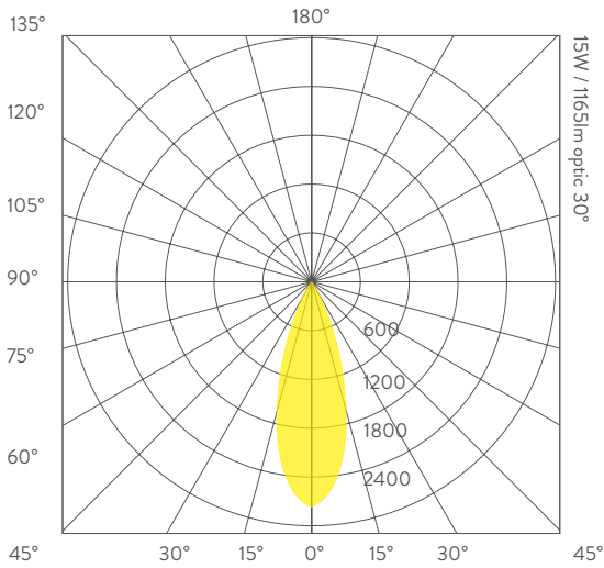
UGR LINE
