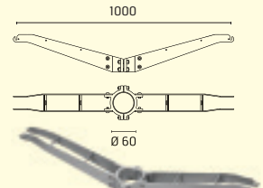
228 DOUBLE BRACKET 500mm FOR POLE Ø 60mm
