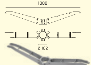
224 DOUBLE BRACKET 500mm FOR POLE Ø 102mm
