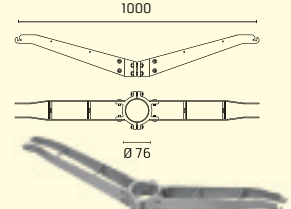
232 DOUBLE BRACKET 500mm FOR POLE Ø 76mm
