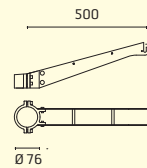
113 SINGLE BRACKET 500mm FOR POLE Ø 76mm
