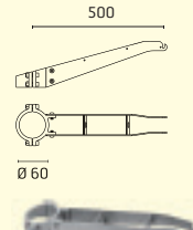
227 SINGLE BRACKET 500mm FOR POLE Ø 60mm
