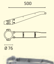
231 SINGLE BRACKET 500mm FOR POLE Ø 76mm
