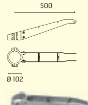
223 SINGLE BRACKET 500mm FOR POLE Ø 102mm
