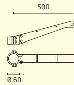
94 SINGLE BRACKET 500mm FOR POLE Ø 60mm
