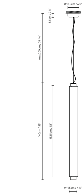
SLIM SKIN SV 1400
