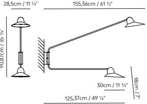
SPEERS ARM W BODY 2 + SHADE L
