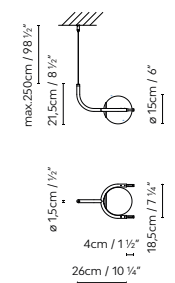
C_BALL S SINGLE SUSPENSION
