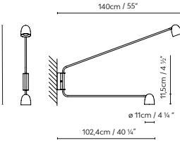
SPEERS ARM W BODY 2 + SHADE S
