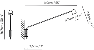
SPEERS ARM W BODY 2 + SHADE S
