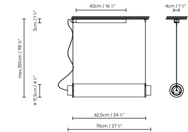
SLIM SKIN SH 700
