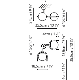
C_BALL SYSTEM C/W 90°H CURRENT SUPPLY
