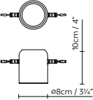
KUPETZ XS POWER SUPPLY
