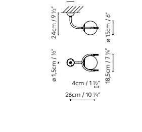
C_BALL SYSTEM C/W CURRENT SUPPLY
