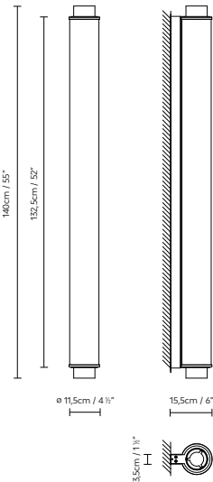
SLIM SKIN W1400
