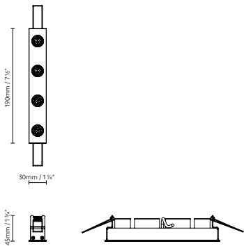
BLOKINLINE MODULE 2 RECESSED
