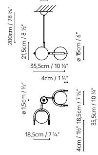
C_BALL SYSTEM C/W CURRENT SUPPLY
