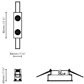
BLOKINLINE MODULE 2 RECESSED
