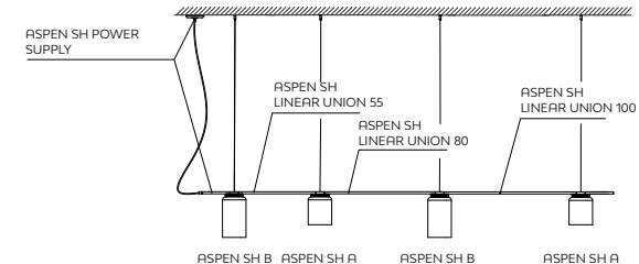
ASPEN SH INSTALLATION EXAMPLE
