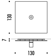
CEILING ROSE
