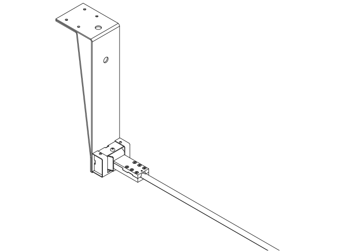
1A0080400.00.00 - Ceiling connection kit
