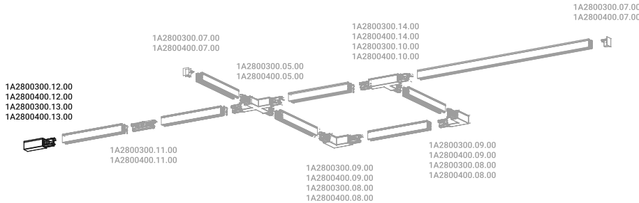
Power right connector and power left connector installation
