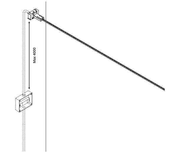
Remote power supply kit
