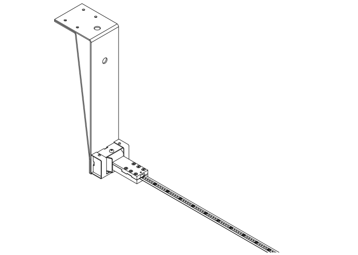
1A0080400.00.00 - Ceiling connection kit
