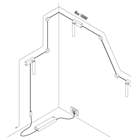
Installation with Endless and Power kit with plug
