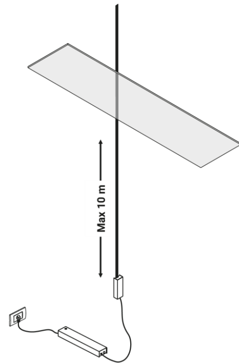
Installation with Endless and Endless Power kit with plug
