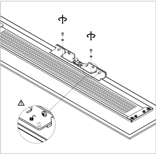
Adjustment A
