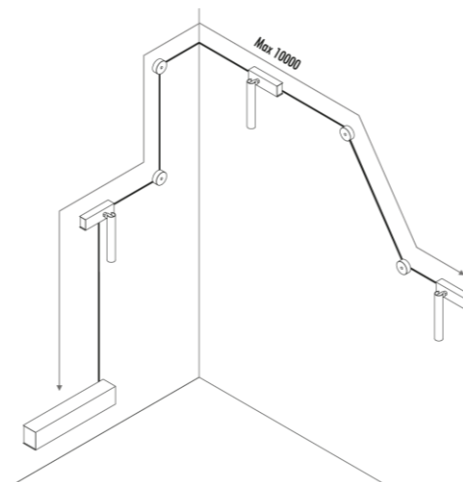
Installation with Endless and Wall-Ceiling rose
