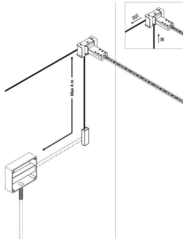
Installation with Endless and Endless Remote Driver
