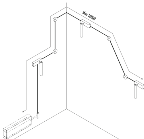
Installation with Endless and Remote Driver
