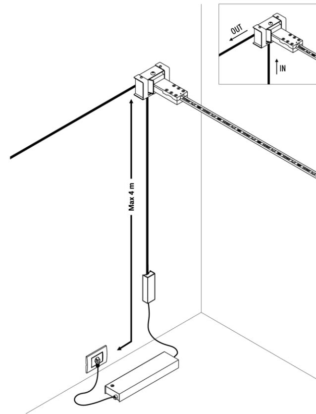
Installation with Endless and Endless Power kit with plug
