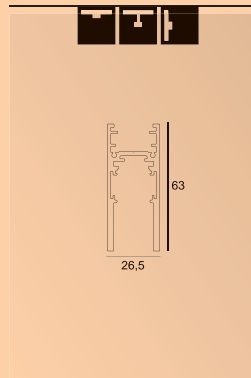
SHIFTLINE M26H
