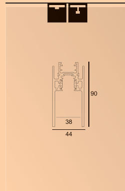
SHIFTLINE M44
