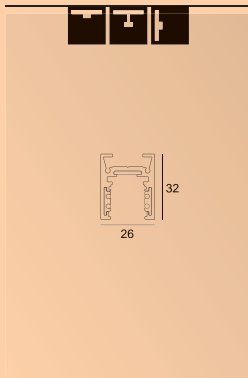
SHIFTLINE M26L
