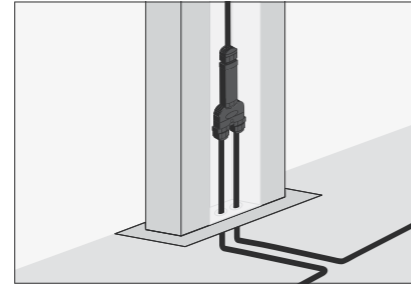
Y-Verbinder: Y-connector:
