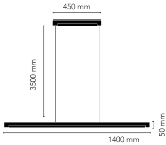
INLAY S1400 LINEAR 13.3W LED - 220-240V Page 54
