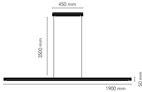
INLAY S1900 LINEAR 2x16W LED - 220-240V Page 54
