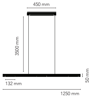
INLAY S1250 LINEAR DISC NEW 3x8W LED - 220-240V Page 52
