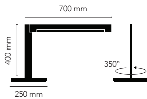
INLAY T2 15W LED - 220-240V Page 58
