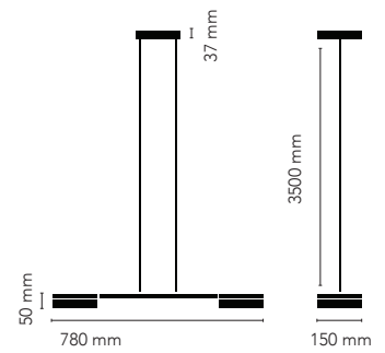
BLADE S2 SLIM 2x16W LED - 220-240V Page 30
