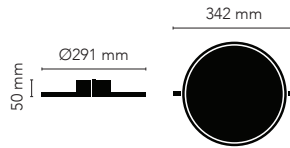
INLAY C2 DISC 18W LED - 220-240V Page 48
