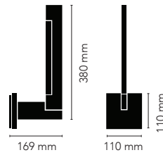
INLAY W2 9W LED - 220-240V Page 56
