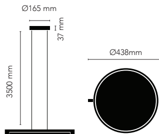
INLAY S3 Ø438 DISC NEW 25W LED - 220-240V Page 50
