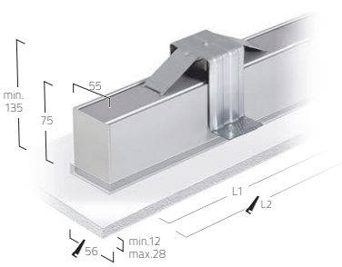
Installation Bracket without Shadow Gap
