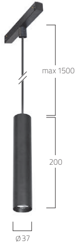
Midpin-C3 Suspended Version
