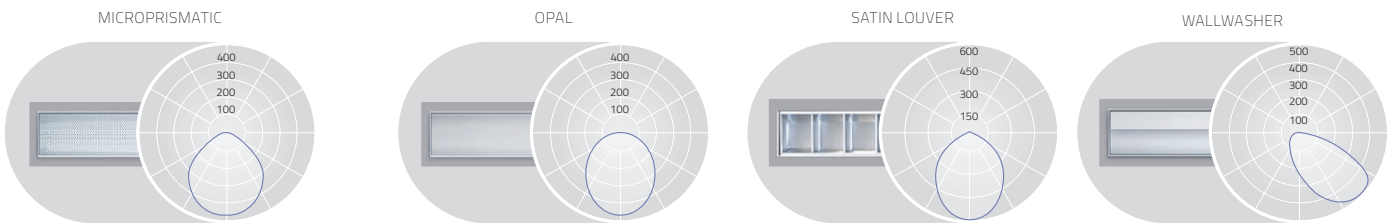
UGR \leq 19 for Low Power (X=4H, Y=8H, S=0.25H) DIRECT 100%
