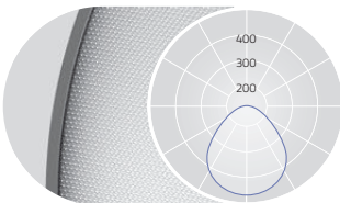
UGR<sub>s19</sub> for Low Power (X=4H, Y=8H, S=0.25H) DIRECT: 100%
