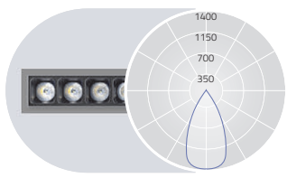
UGR<16 (X=4H, Y=8H, S=0.25H) DIRECT: 100%
