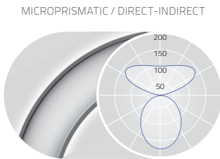
UGR \leq 19 for Medium Power (X=4H, Y=8H, S=0.25H) DIRECT: ca.40% INDIRECT ca.60%
