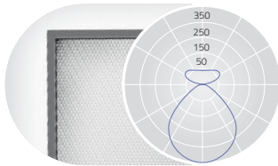
UGR≤19 (X=4H, Y=8H, S=0.25H) DIRECT: ca.75% INDIRECT ca.25%
