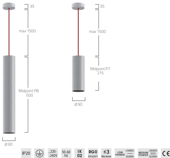
SPOT 10° LED ENGINE ECO, MEDIUM POWER
