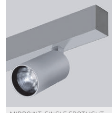
MIDPOINT-SINGLE SPOTLIGHT Max. 3000lm/30W/ \varnothing 90 mm
