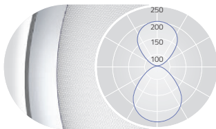
UGR 16 (X=4H, Y=8H, S=0.25H) DIRECT: ca.50% INDIRECT ca.50%
