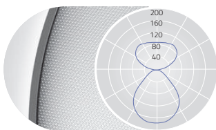
UGR s 19 (X=4H, Y=8H, S=0.25H) DIRECT: ca.55% INDIRECT ca.45%
