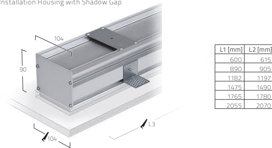
Installation Housing with Shadow Gap
