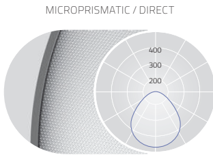
UGR \leq 19 for Low Power (X=4H, Y=8H, S=0.25H) DIRECT: 100%
