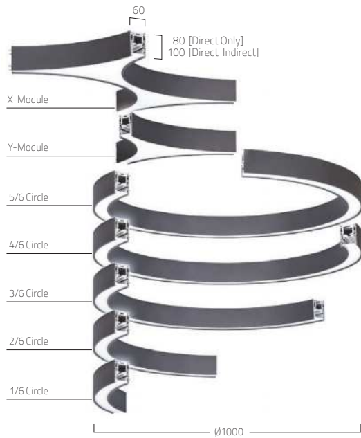
OPAL DIFFUSER / DIRECT-INDIRECT
