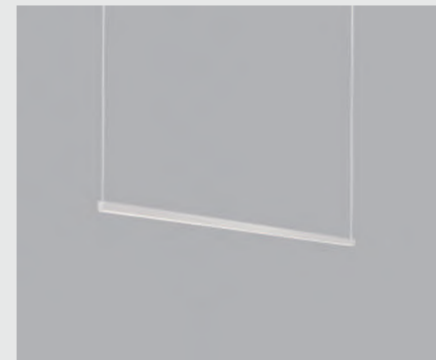
STRIPE S1500 / White / ART. No 270360 Design: Ronni Gol 1x27W LED - 230V - IP20 indoor only CRI > 90 - 2700K - Dimmable Dimensions: 1500 x 15 mm
