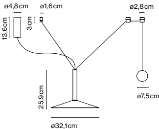
Milana 32 Counterweight
