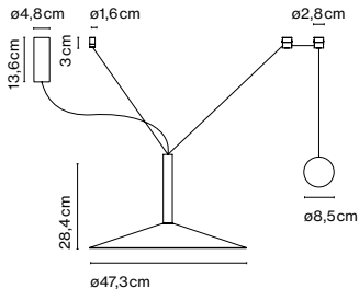
Milana 47 Counterweight
