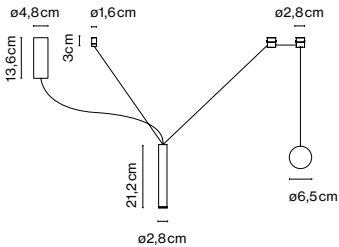
Milana Counterweight
