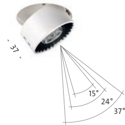
LED 8,4 W / 700 mA spot 15° CAL/KLM
