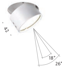
HIT spot 18° CAL/KLM
