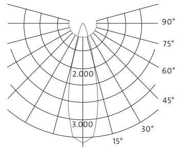
LED 8,4 W / 700 mA medium 24° CAL/KLM
