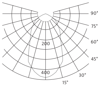
NV flood 45° (35W) CAL/KLM
