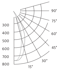
HIT flood 26° CAL/KLM
