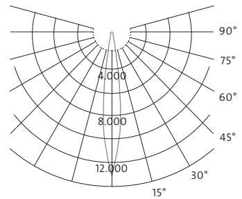
LED 8,4 W / 700 mA spot 15° CAL/KLM
