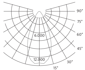
LED 8,4 W / 700 mA flood 37° CAL/KLM
