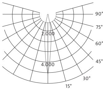
NV flood 15° (35W) CAL/KLM
