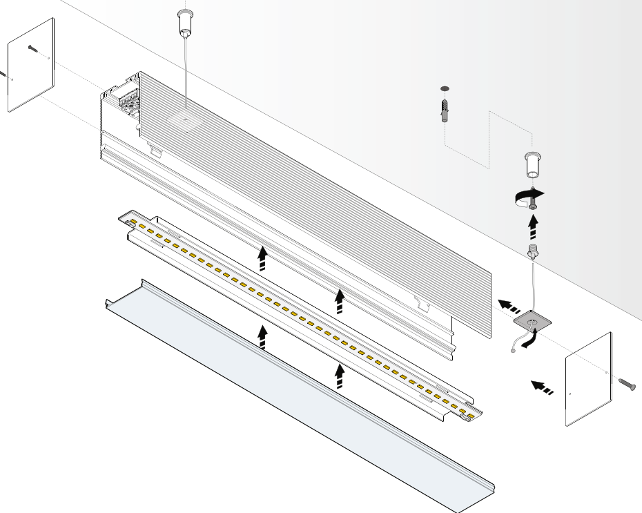
XG2038-U90 XP Giunzione piana 90° con LED e driver Level junction 90° with LED and driver
