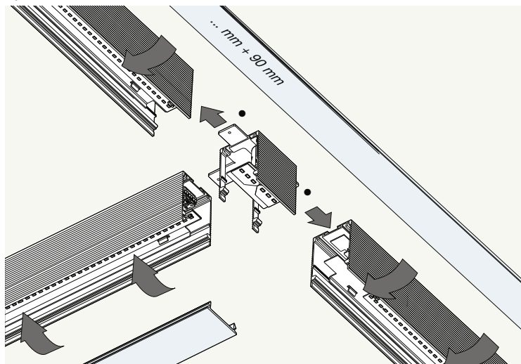
XG2038-UT Giunzione a T con LED e driver T junction with LED and driver
