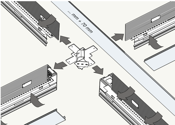
XG2038-X Giunzione a X trimless con LED e driver X junction trimless with LED and driver
