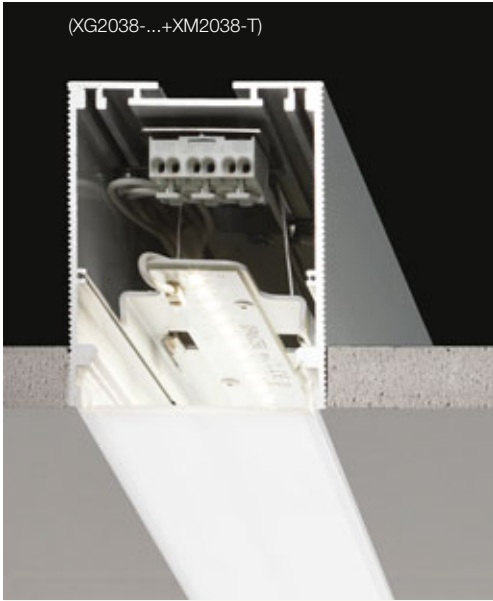
XG2038 TRIMLESS PROFILE
