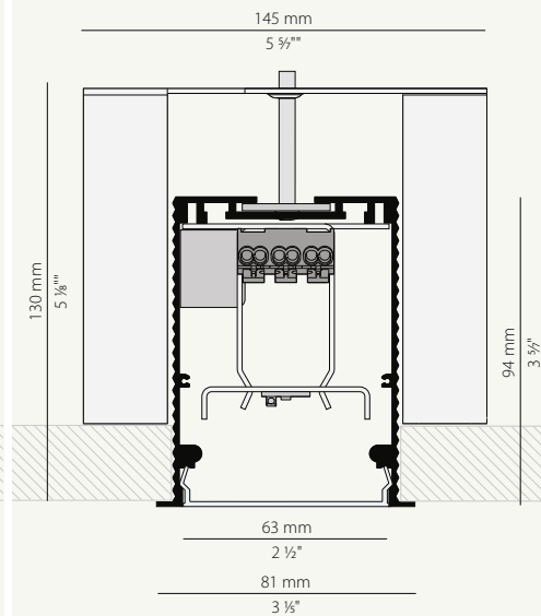
XG2039 TRIM PROFILE
