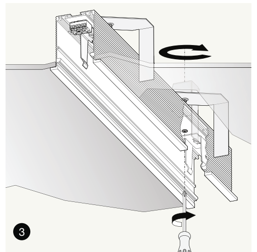
XG2039-U90 Giunzione piana 90° trim con LED e driver Level junction 90° trim with LED and driver
