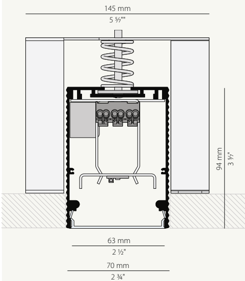
XG2038 TRIMLESS PROFILE
