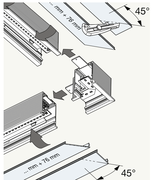
XG2039-U90 Giunzione piana 90° trim con LED e driver Level junction 90° trim with LED and driver
