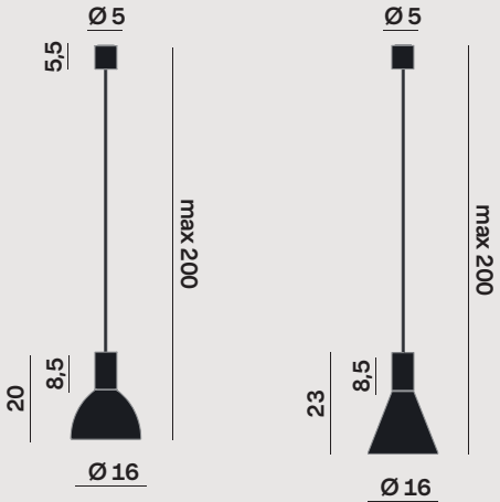
Pendant spotlight with glass reflector on cord
