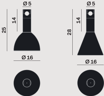
Track spotlight with glass diffuser
