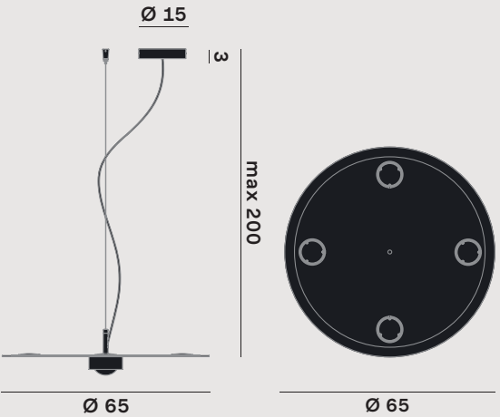
Collide H6 D
