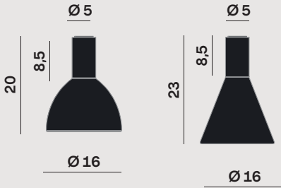
Ceiling mounted spotlight with glass reflector*
