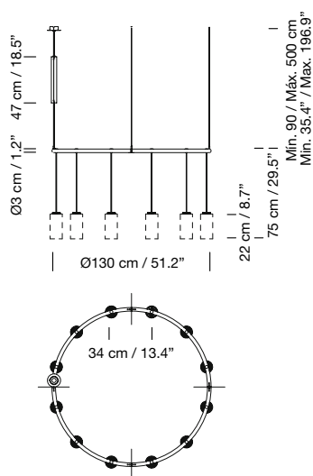
Circular canopy
