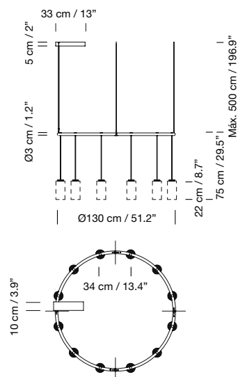
Rectangular canopy
