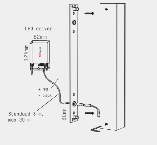
FIX / External model
