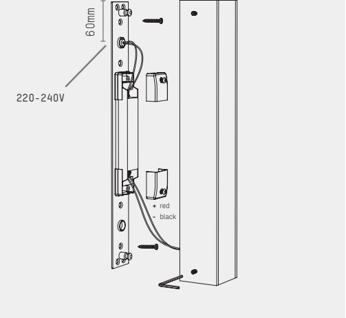
FIX / Built-in model
