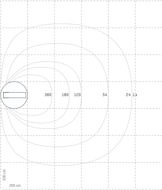
Led 40 table lx
