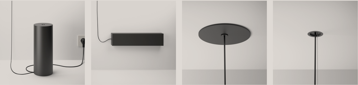
Floor base & plug ø 13x32 cm Surface canopy 40x4x10 cm Built-in disc S ø 12x6 cm Remote driver Built-in Micro ø 4x7 cm
