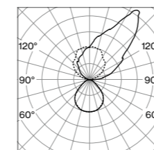
microprismatic direct/indirect power
