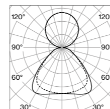
microprismatic direct/indirect
