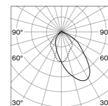
SPADO 150 asymmetric
